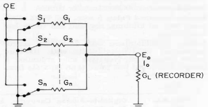
Figure 4. Equivalent circuit of the output matrix.
