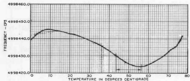
Figure 2. Frequency-vs-temperature characteristic of 5-Mc crystal. Full scale for analog curve was 100 cps, each minor division 1 cps. Only the significant part of the analog record (from 4998420.0 to 4998460.0) is reproduced here. Gate time was 10 seconds.
