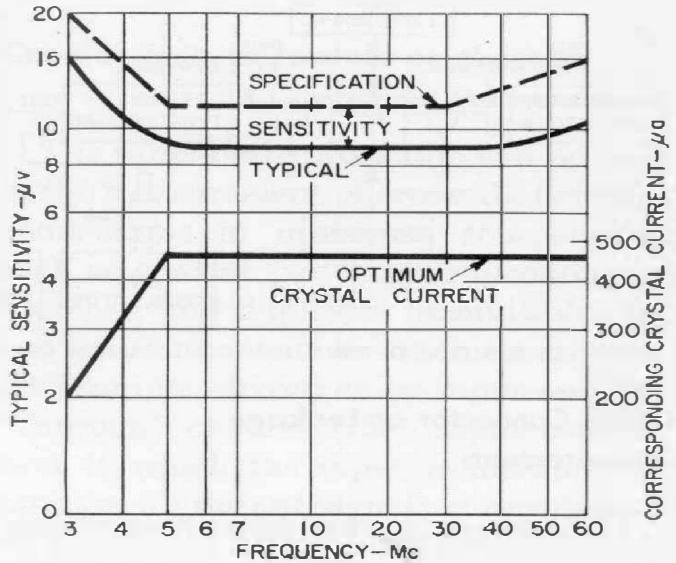
Figure 12. Sensitivity vs frequency.
