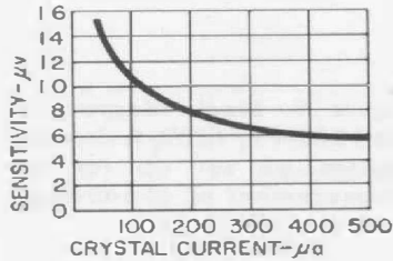
Figure 11. Sensitivity (open-circuit voltage from 50-ohm source, for 1% meter deflection) vs local-oscillator drive for the 1212-P3/1212-A detector system.
