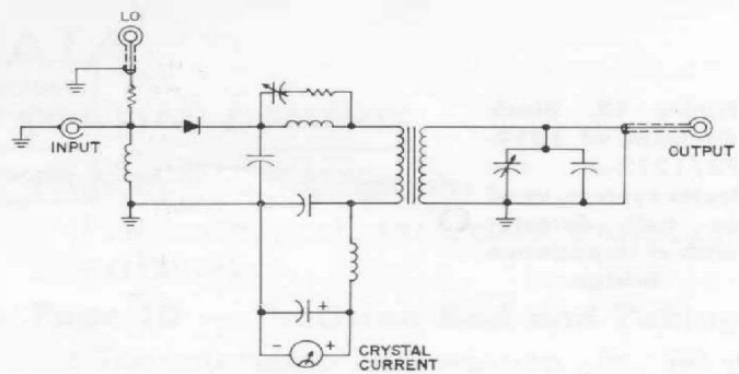
Figure 10. Schematic of the Type 1212-P3 RF Mixer.
