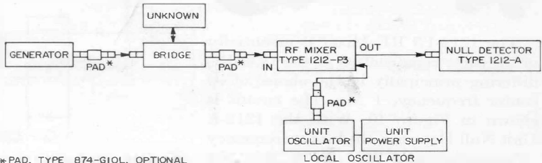
Figure 13. Block diagram of 1212-P3/1212-A detector system, used as null detector with rf impedance bridge.
