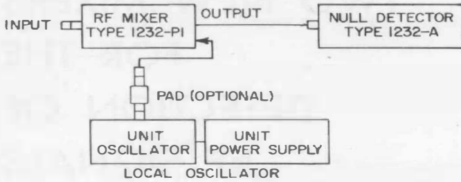
Figure 2. Block diagram of complete detector system using the Type 1232-P1 RF Mixer.
