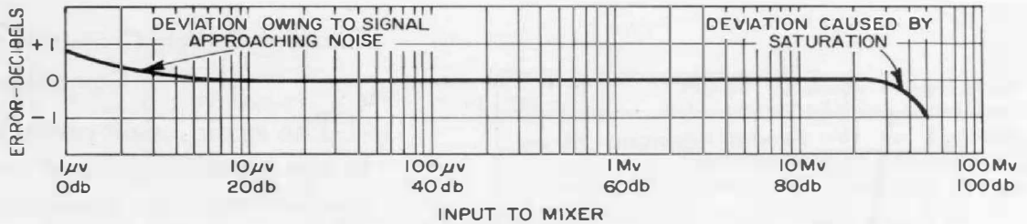
Figure 4. Linearity of the 1232-PL/1232-A detector as a function of input voltage.
