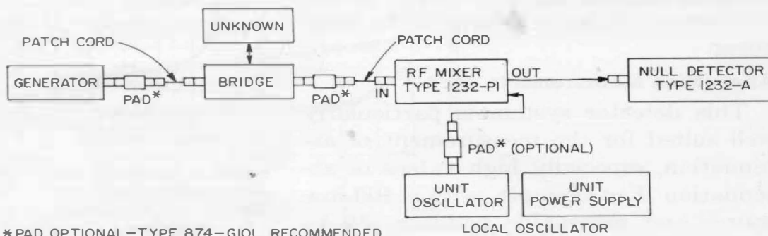
Figure 8. Block diagram of the detector system used as a bridge null detector.
