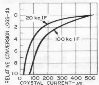
Figure 6. Relative conversion loss vs local-oscillator drive.
