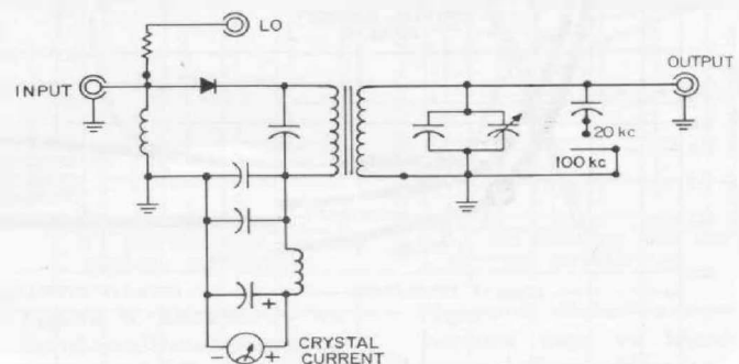
Figure 1. Schematic diagram of the mixer circuit.
