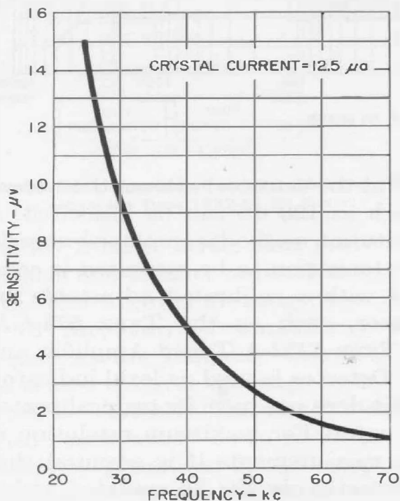
Figure 7. Typical sensitivity at frequencies below normal range.
