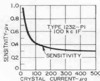
Figure 5. Sensitivity vs local-oscillator drive for 100-kc intermediate frequency.
